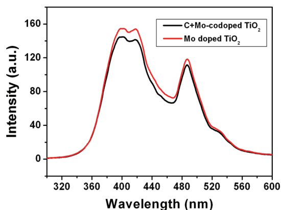
Figure 8. PL spectra of Mo-doped \text{TiO}_2 and C + Mo-codoped \text{TiO}_2 .
