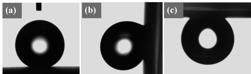
Figure 4. Shapes of the water droplets on the lotus-leaf-like ZnO micromonanostructure films at tilt angles of (a) 0°, (b) 90°, and (c) 180°.
